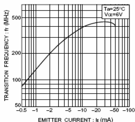
Fig.6 Gain bandwidth product vs. emitter current
